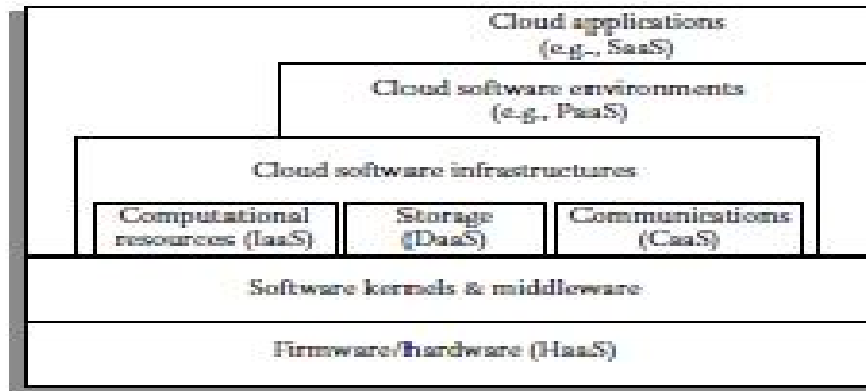
Figure 2: UCSB-IBM Cloud Ontology
